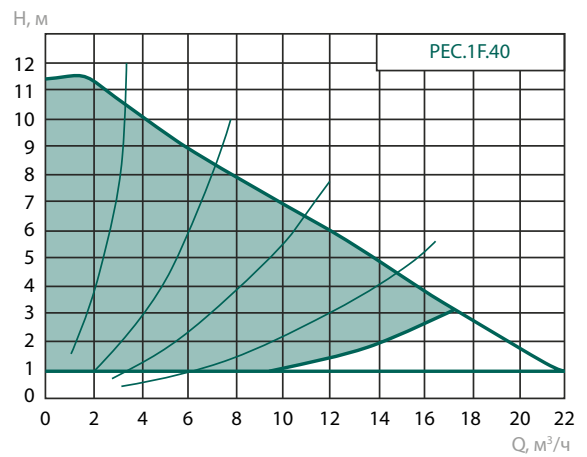
PEC.1F.40 / PEC.3F.50 / PEC.3F.80
